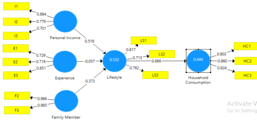
Figure 2: PLS Analysis
